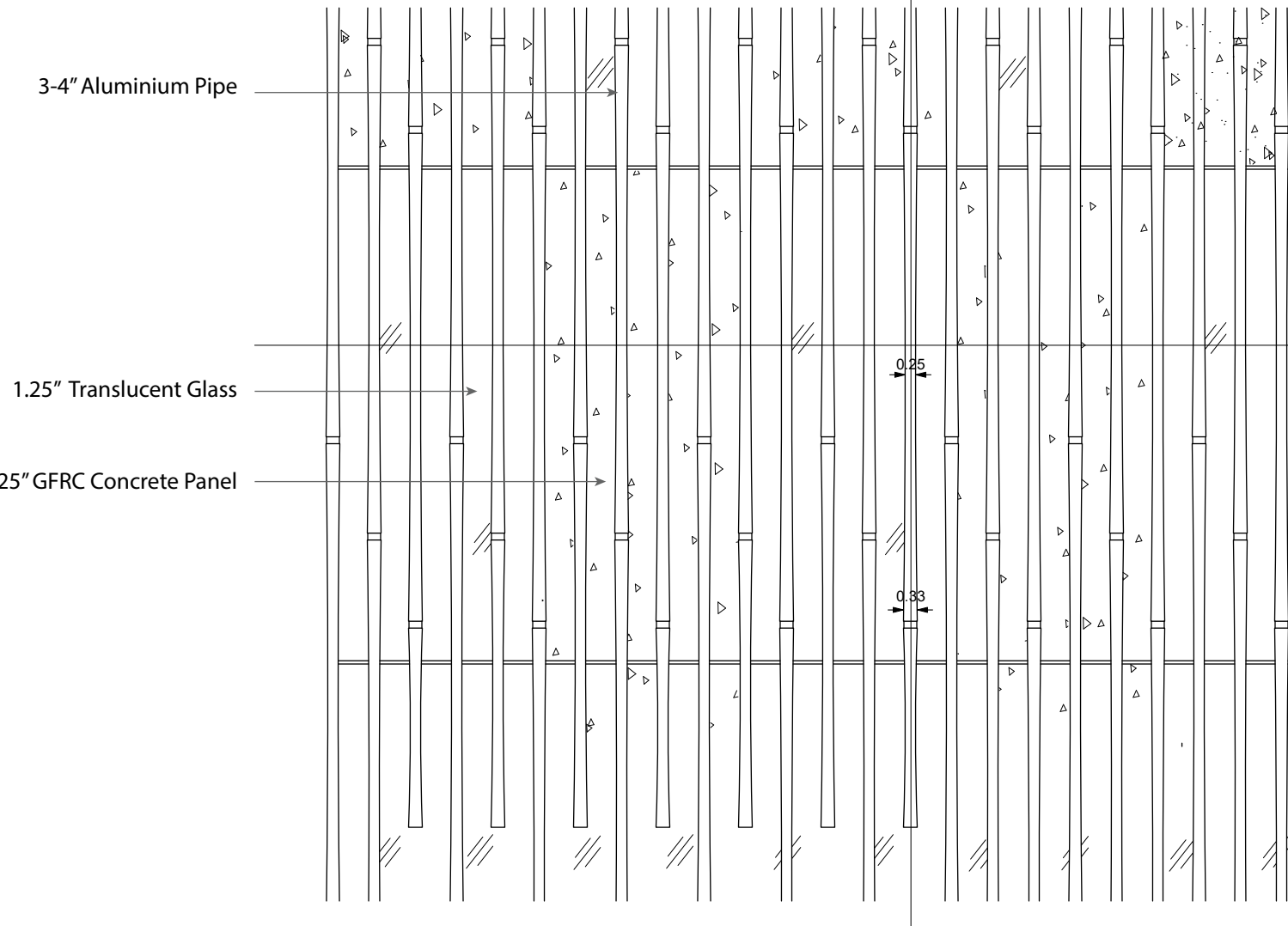
Typical Elevation 1/4" = 1' - 0"
