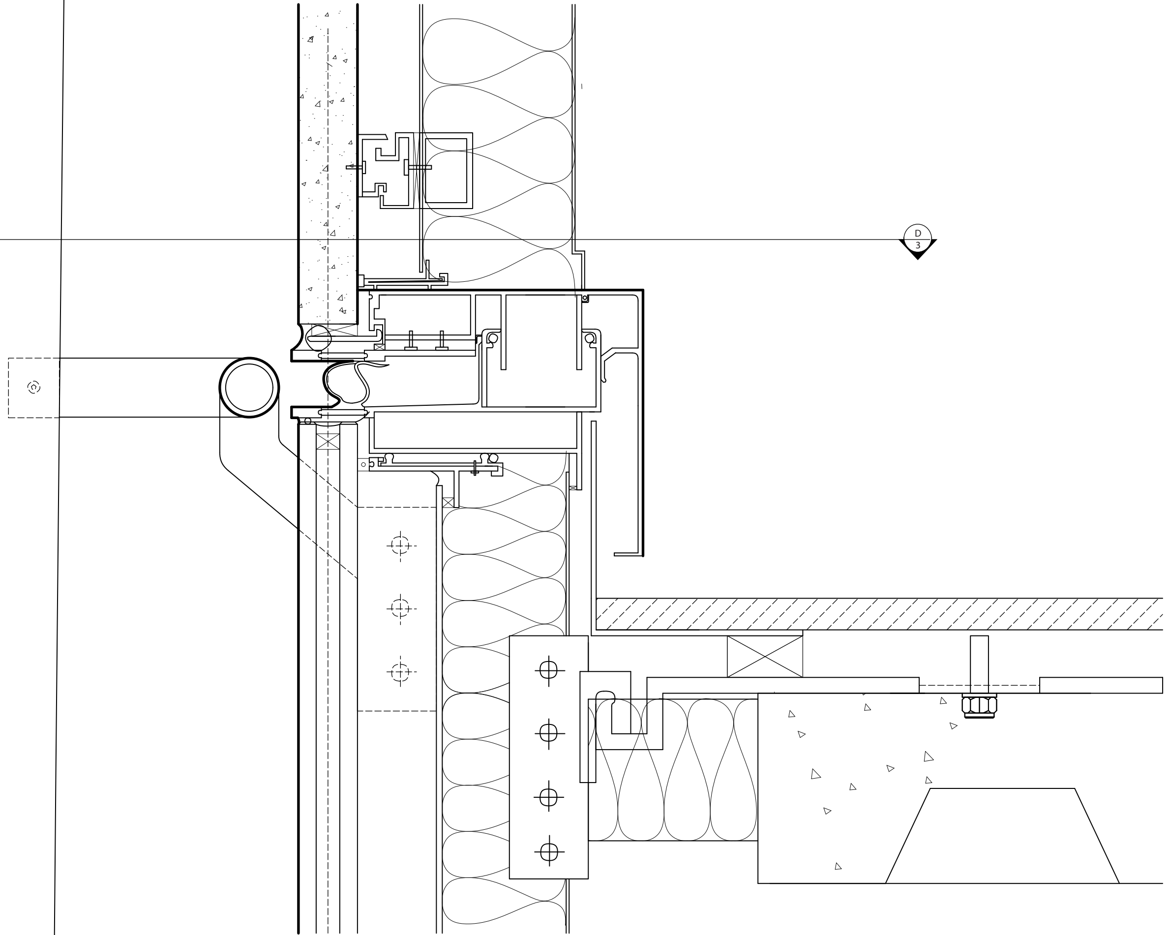
C2 Mullion Typical Section Detail 6" = 1'-0"
