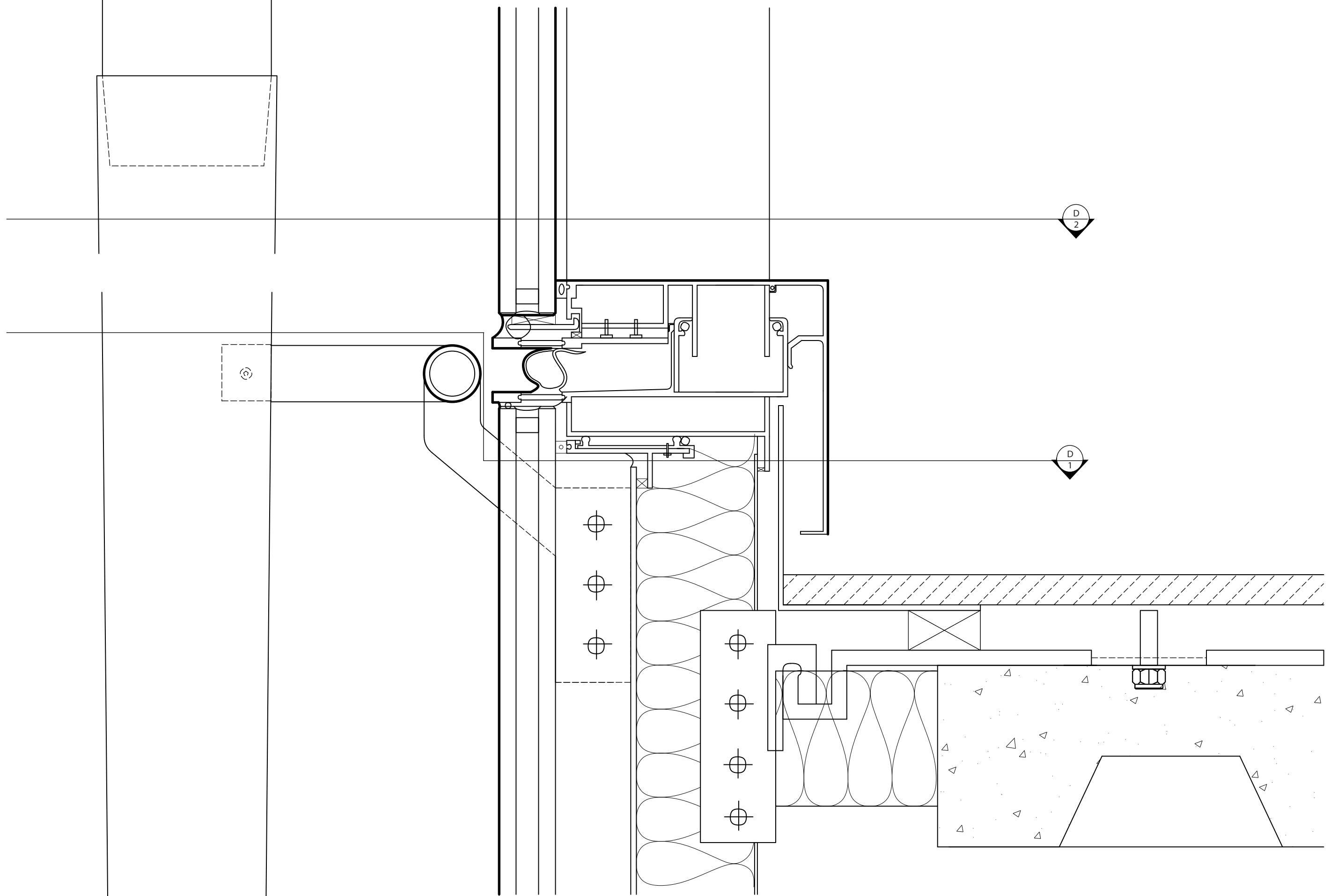
C1 Mullion Typical Section Detail 6" = 1' - 0"
