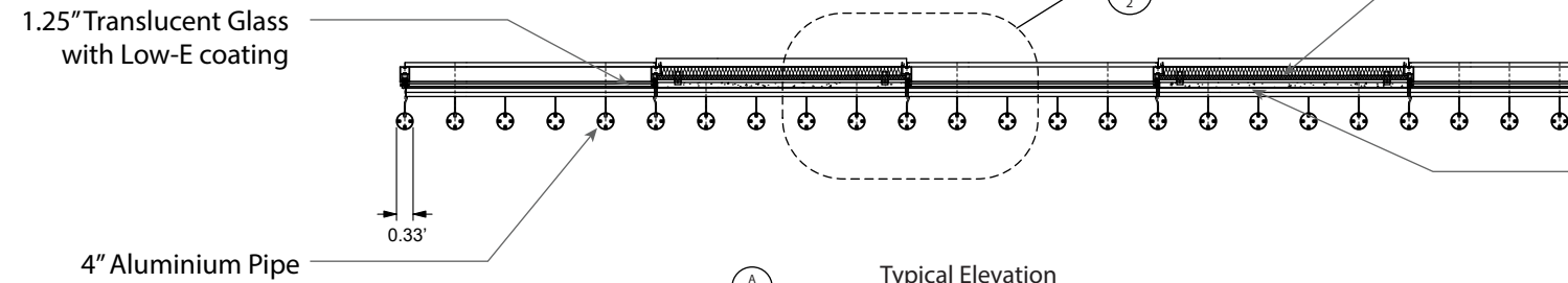
Typical Elevation 1/4" = 1' - 0"
