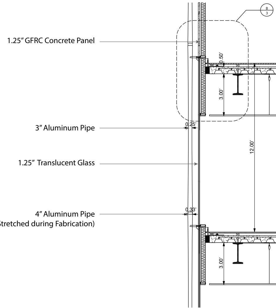
Typical Section 1/4" = 1' - 0"
