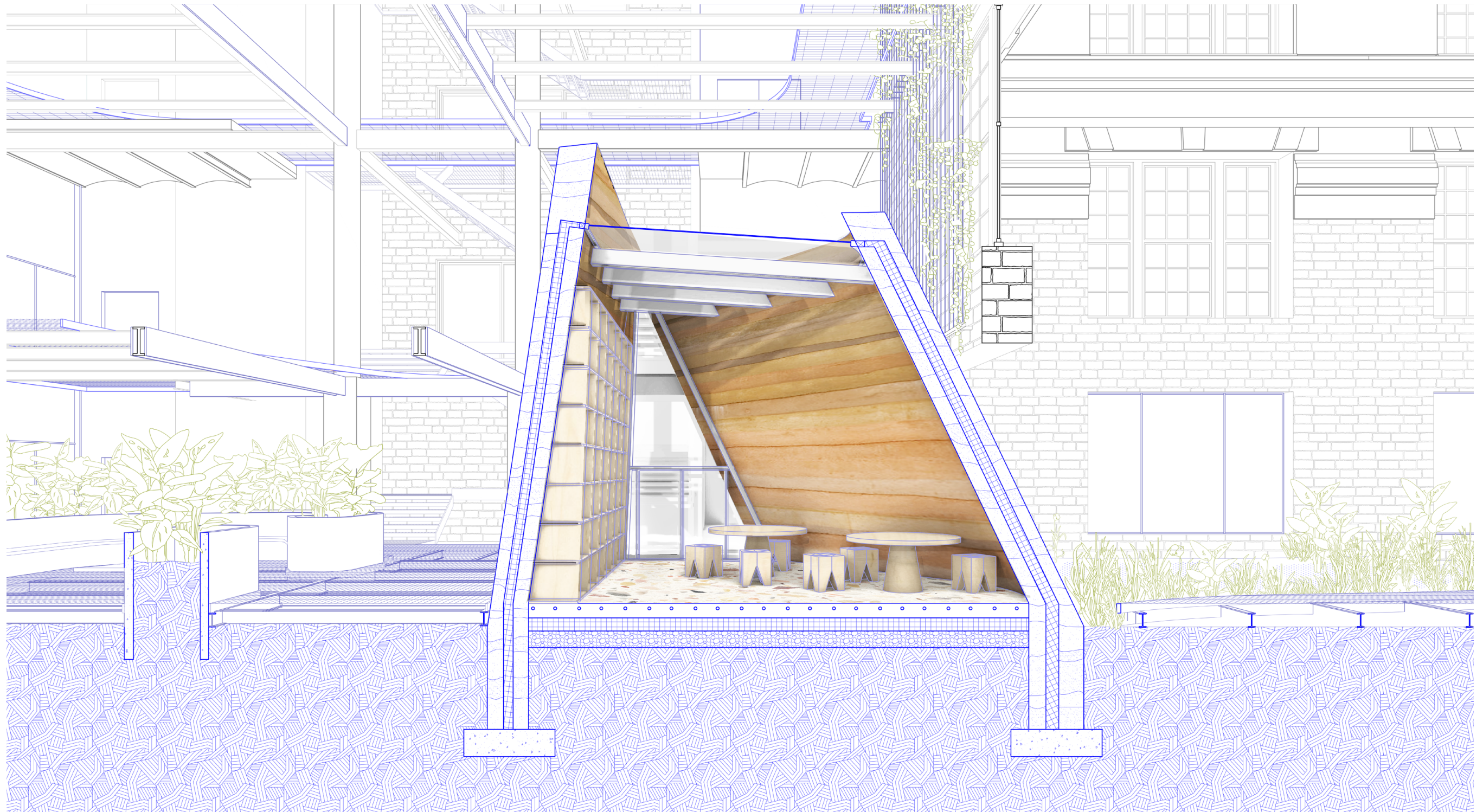
Geology Pod Detail
