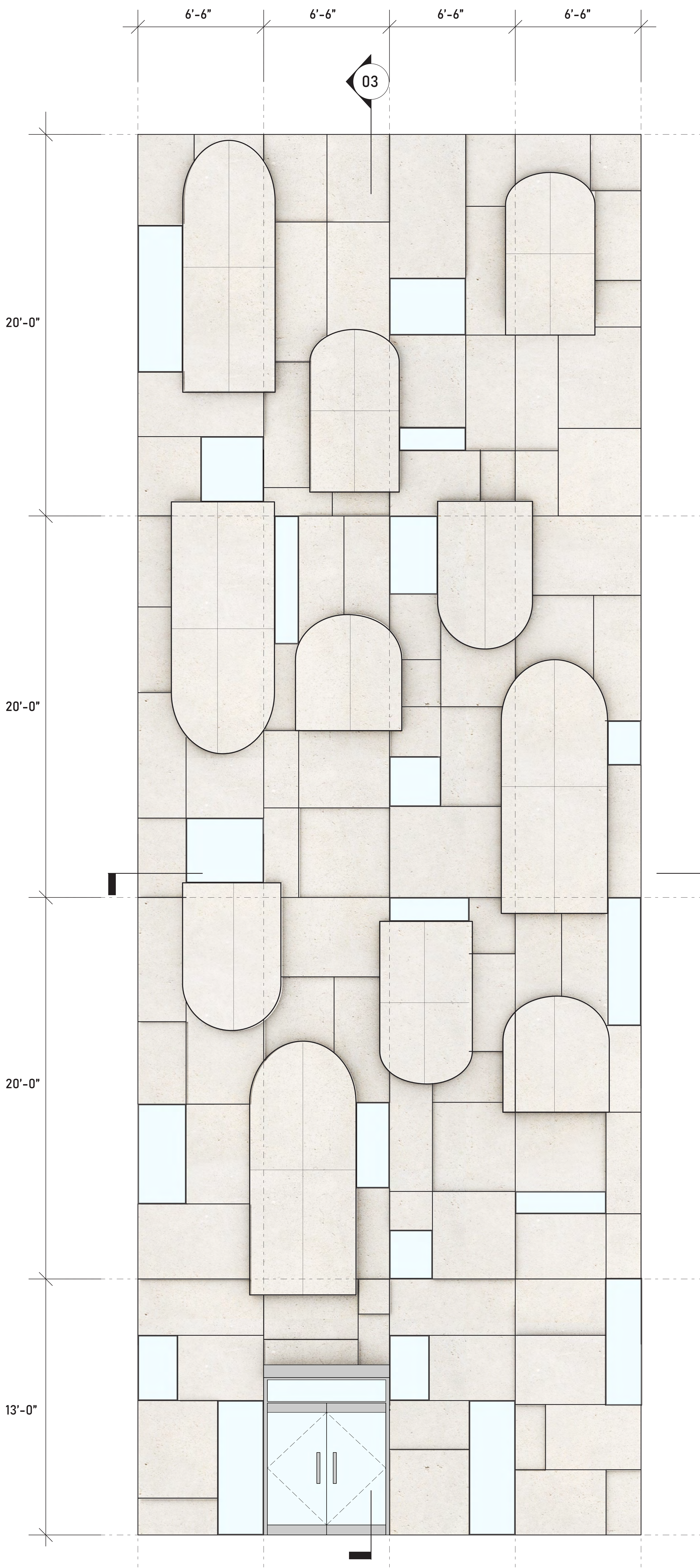
01 Elevation - Full Facade 1/2" = 1'-0"
