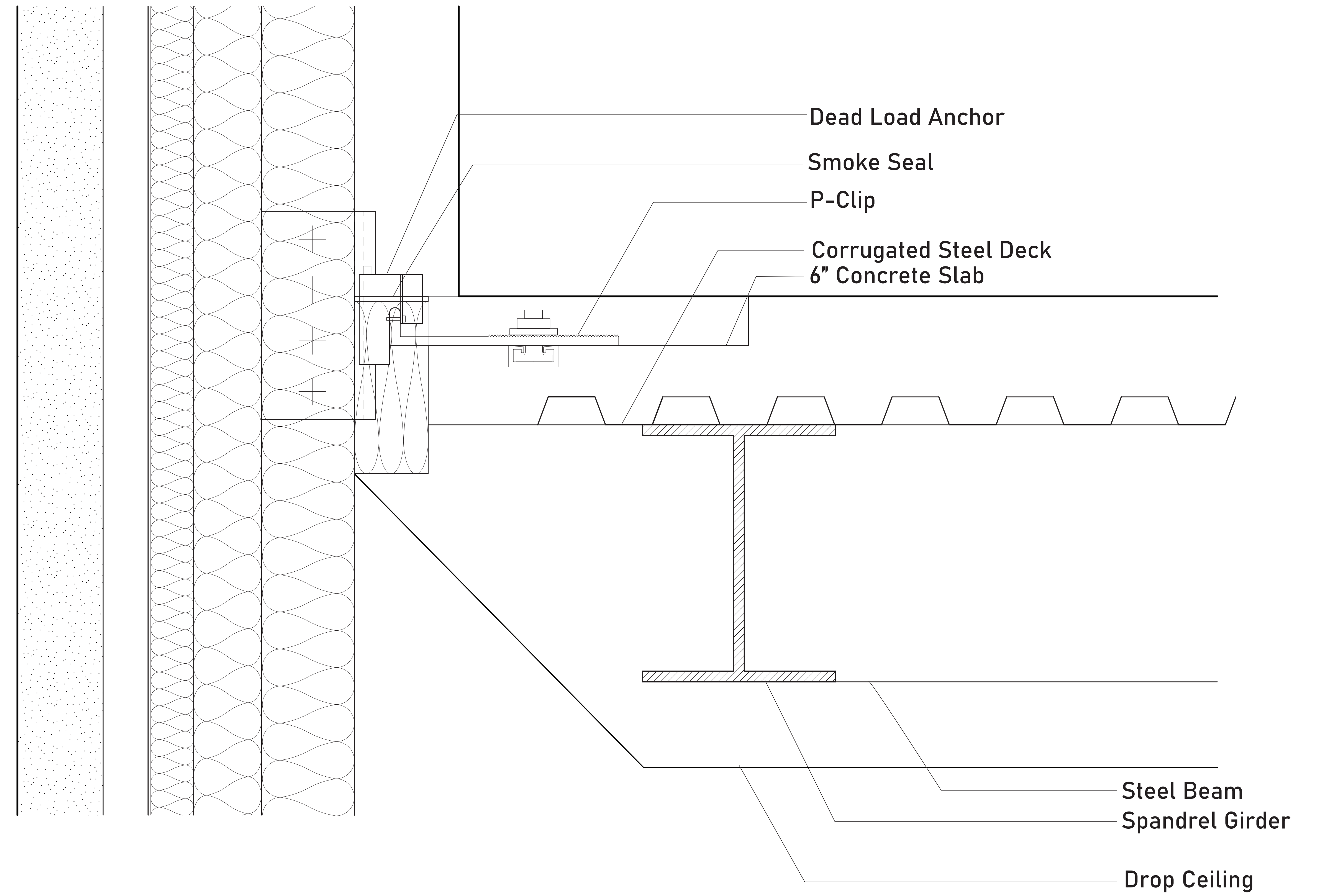
D2 Section - Mullion to Floor Connection 3" = 1'-0"
