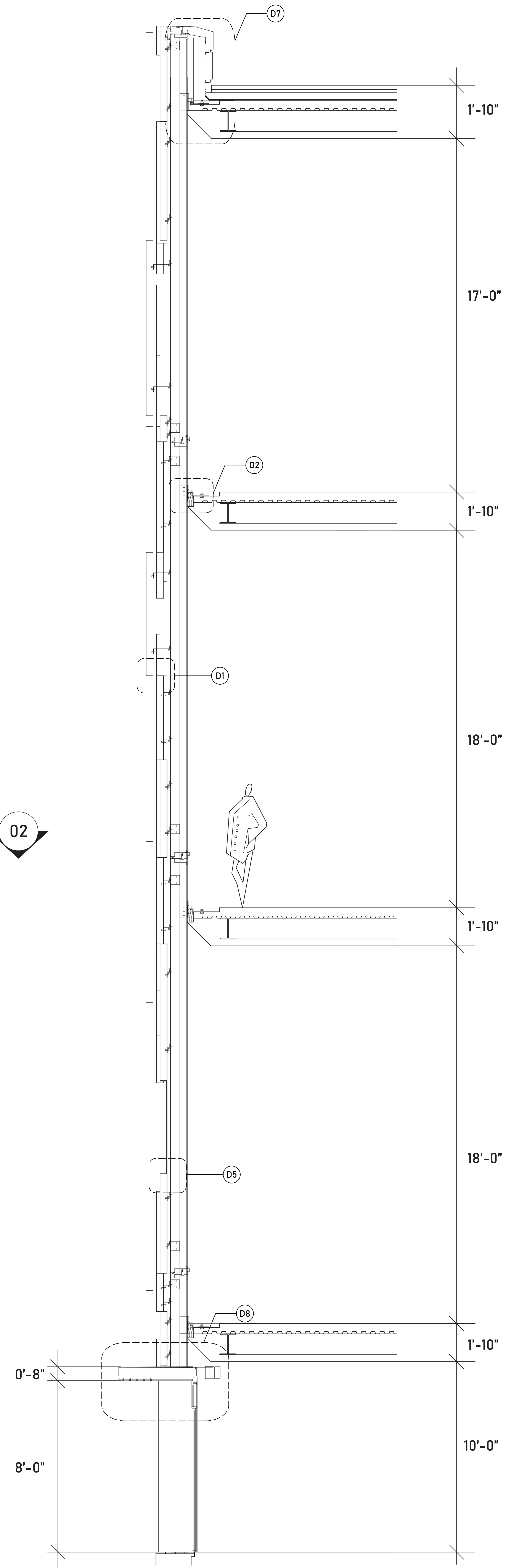
03 Section 1/2" = 1'-0"
