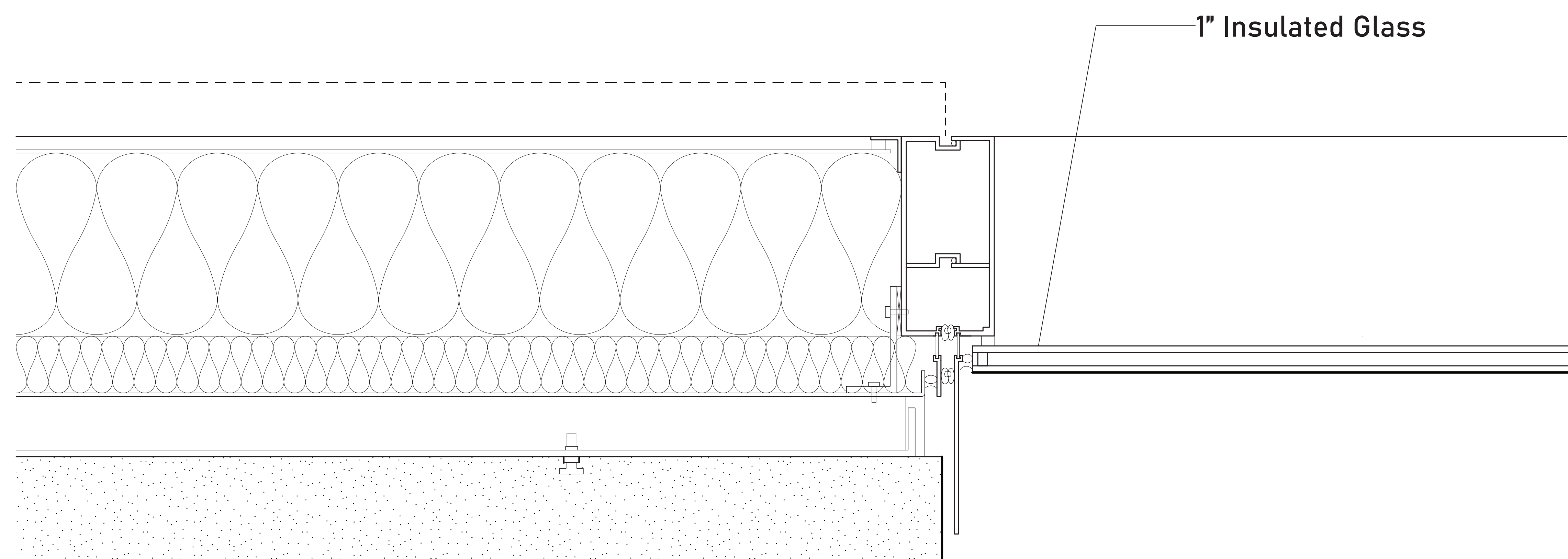
D4 Enlarged Plan - Limestone to Glass Connection 3" = 1'-0"
