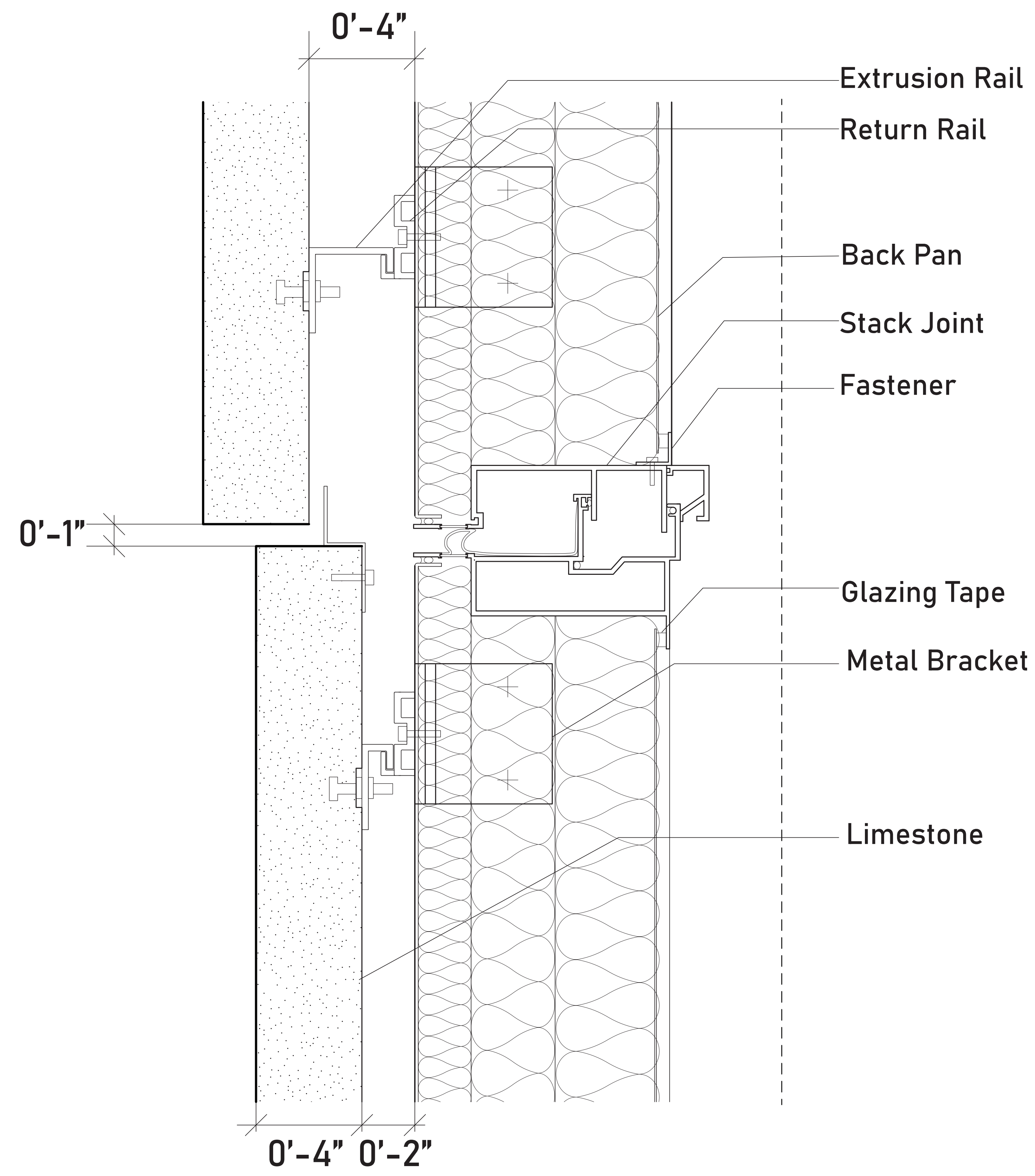
D1 Section - Limestone to Mullion Connection 3" = 1'-0"
