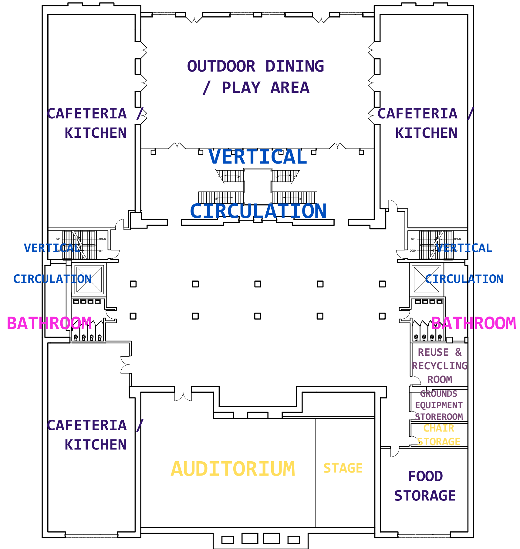
⊗ CELLAR FLOOR PLAN
