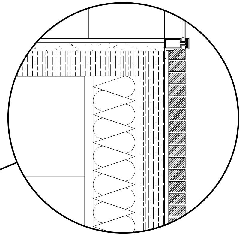
WALL DETAIL
