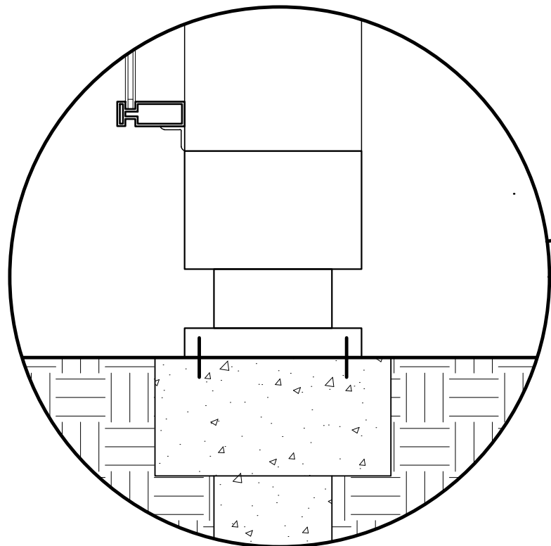
COLUMN TO GROUND CONNECTION
