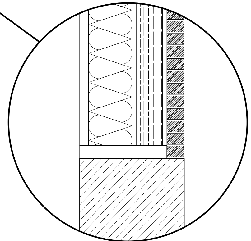
COLUMN & EXTERIOR CLADDING TO EXISTING MASONRY WALL
