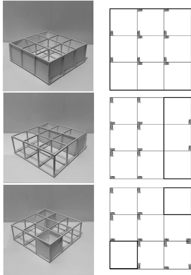
Folding Wall
