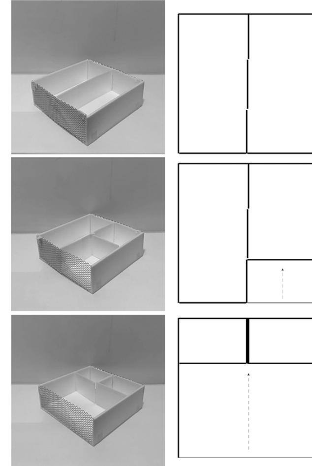
Sliding Wall
