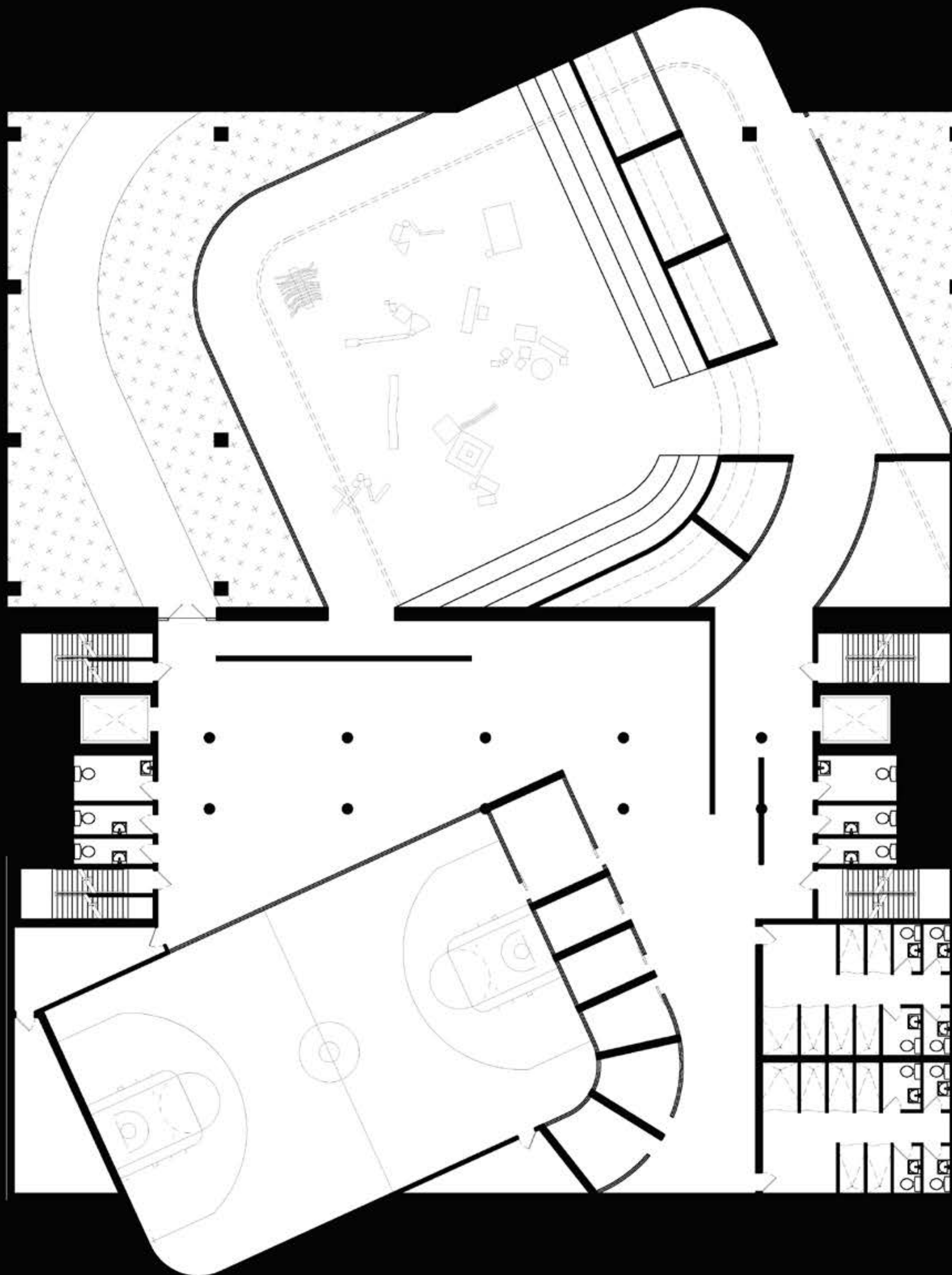
basement plan
