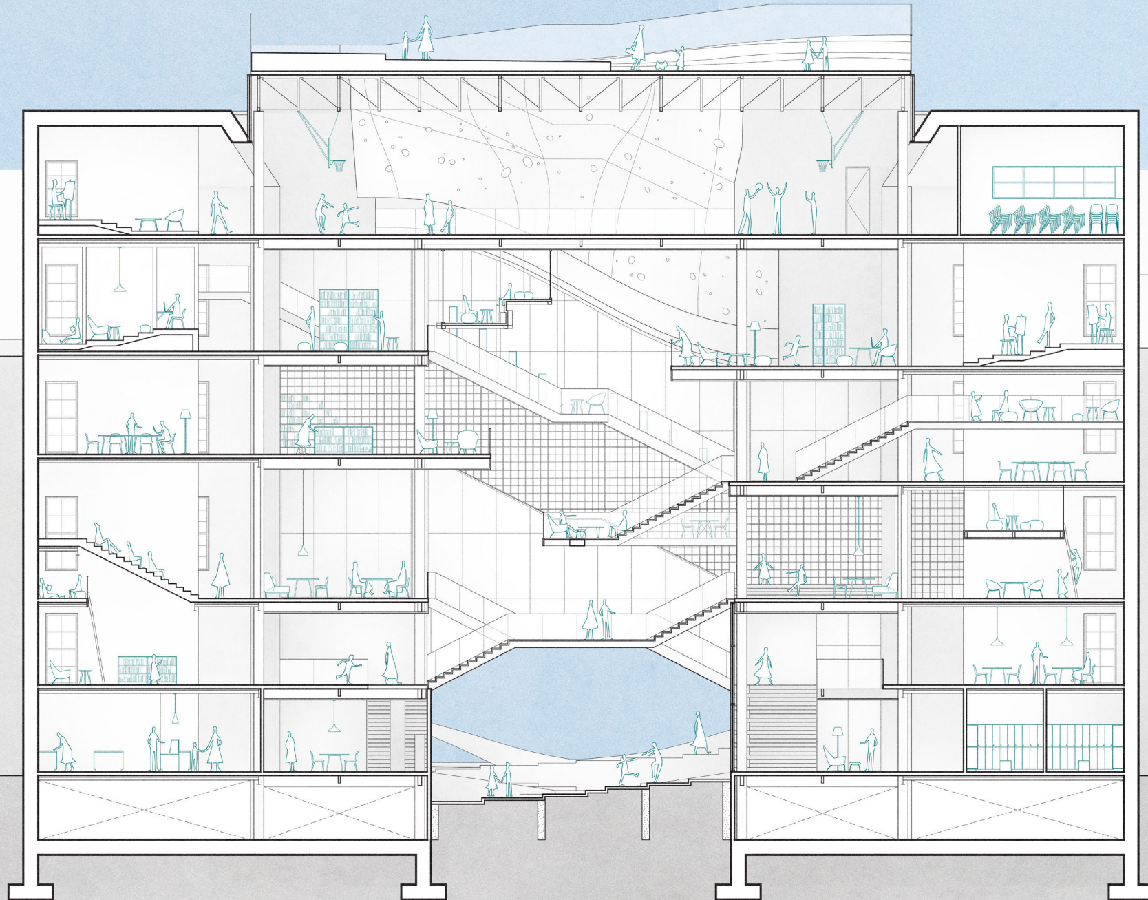
Section
