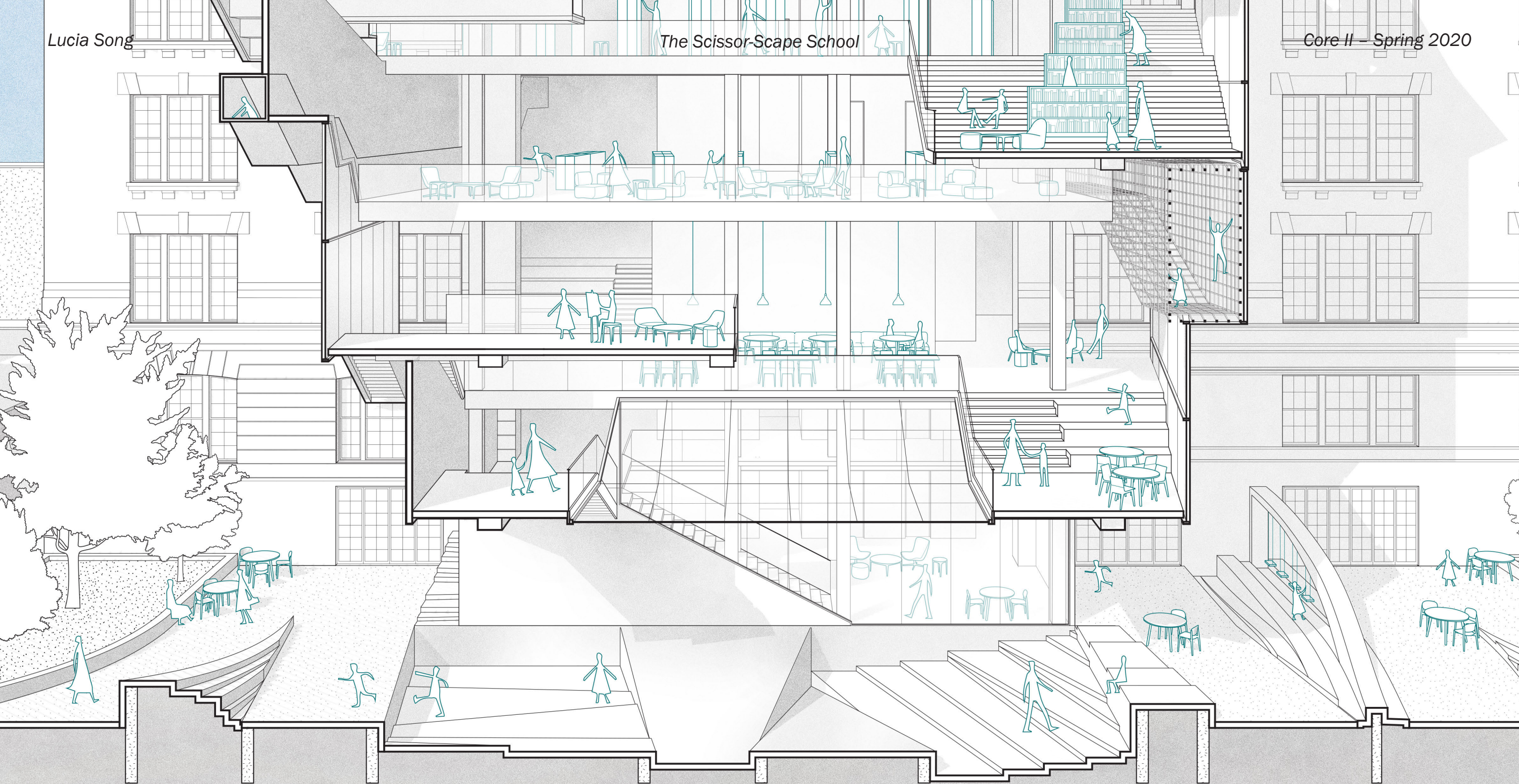
Section Perspective
