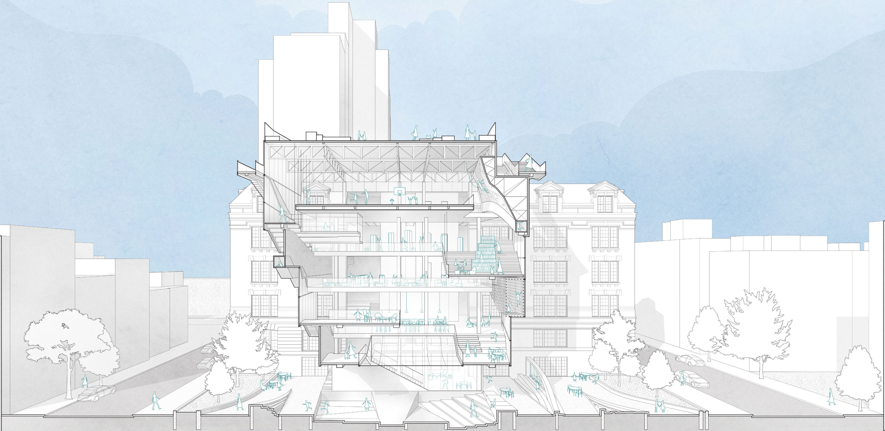
Section Perspective
