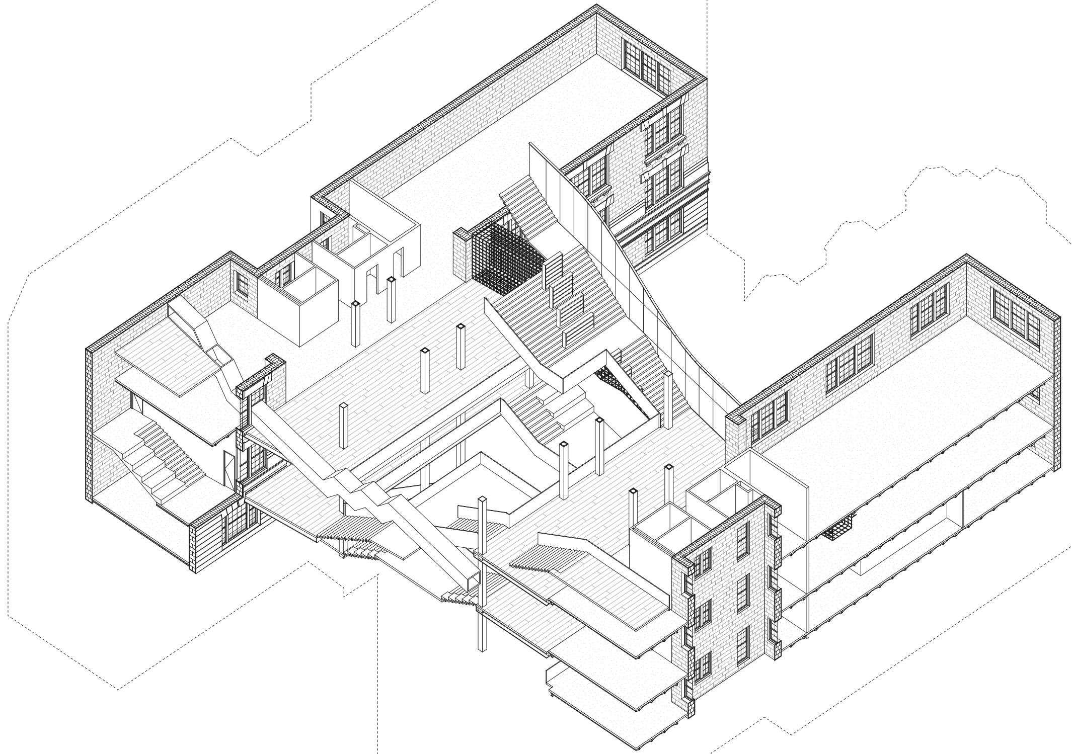
Isometric Cutaway
